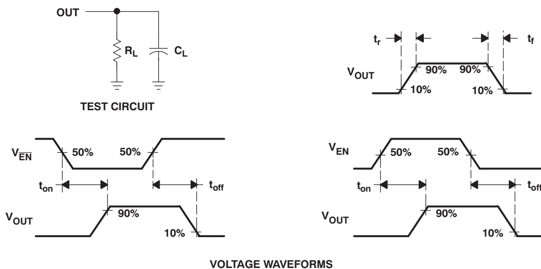
Figure 2. Test Circuit and Voltage Waveforms
